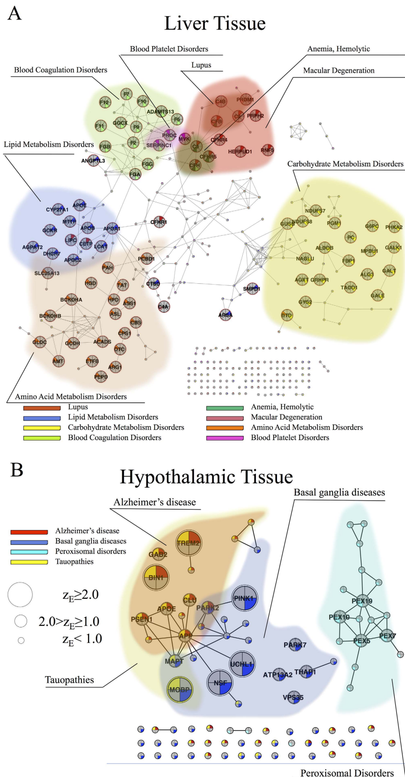
Figure 5. Diseases associated with liver and hypothalamus. (A) Diseases associated with the liver-specific interactome. (B) Diseases associated with the hypothalamus-specific interactome. Node sizes depend on the expression significance of the corresponding genes. We use pie-chart coloring to reflect disease-gene associations. To improve the readability of diagrams, we grouped genes related to the same disease into modules and highlighted each module accordingly. We excluded disease genes associated with nutritional and metabolic diseases from both panels owing to the large number of associated genes.
