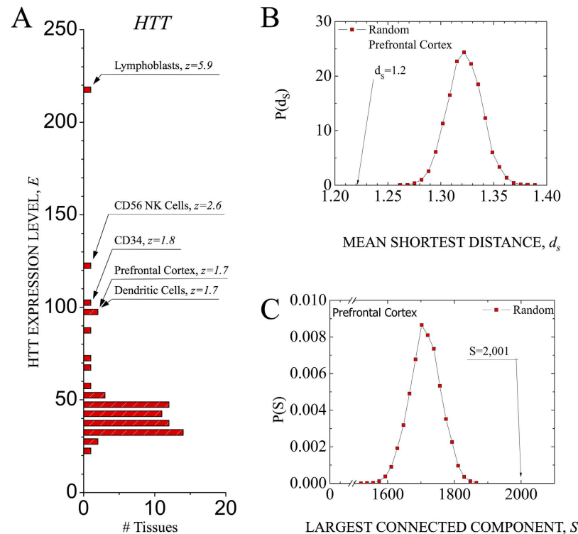
Figure 1. Network-based localization of expressed genes. (A) The distribution of expression levels of the HTT gene across 64 non-diseased tissues. (B) The distribution of the mean shortest distance d_s for randomly chosen sets of genes in the human interactome. The number of randomly selected genes in each set is chosen to match the number of genes expressed in prefrontal cortex at z_E \geq 1.0 . Note that the observed mean shortest distance for genes expressed in prefrontal cortex, d_{s, \text{prefr.cort}} = 1.22 , is significantly lower than the random expectation. (C) The distribution of the connected components size, P(S) , for randomly chosen sets of genes in the human interactome. The number of randomly selected genes in each set is chosen to match the number of genes expressed in prefrontal cortex at z_E \geq 1.0 . Note that the size of the connected component for genes expressed in prefrontal cortex, S_{\text{prefr.cort}} = 2,001 , is significantly greater than the random expectation.
